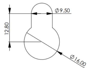
ENLARGED MOUNTING HOLE
