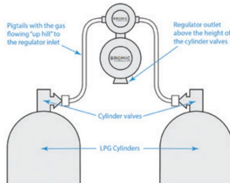
Figure 1. Two cylinders and pigtails connected via manual changeover valve
